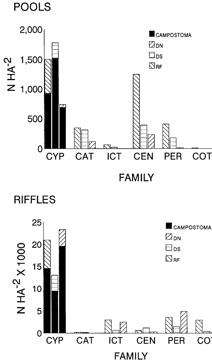
FIGURE 5.—Abundance of families of fish collected from upstream reference (RF), disturbed (DS), and downstream reaches (DN) in pools and riffles of three Ozark streams with the density of central stoneroller Campostoma anomalum indicated. CYP = Cyprinidae, CAT = Catostomidae, ICT = Ictaluridae, CEN = Centrarchidae, PER = Percidae, COT = Cottidae.
