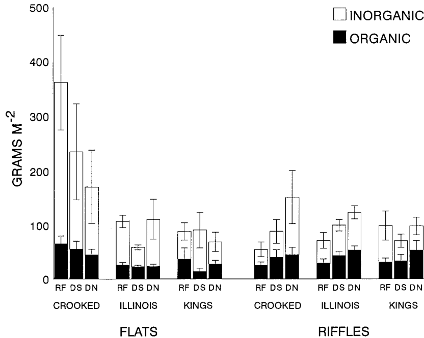
FIGURE 2.—Mass of biofilm on cobbles (64–100 mm) taken from riffles and flats in three Ozark streams in reference (RF), disturbed (DS), and downstream (DN) reaches near large gravel mines. Error bars = \pm 2 SE of means.
